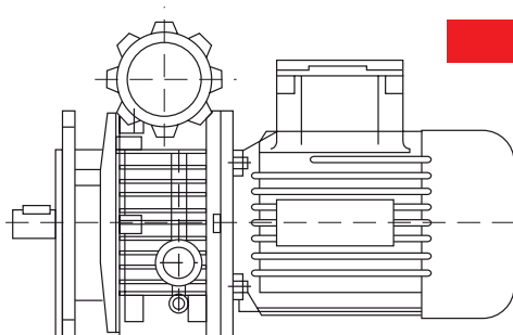
Mounting position
